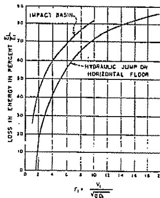
COMPARISON OF ENERGY LOSSES
