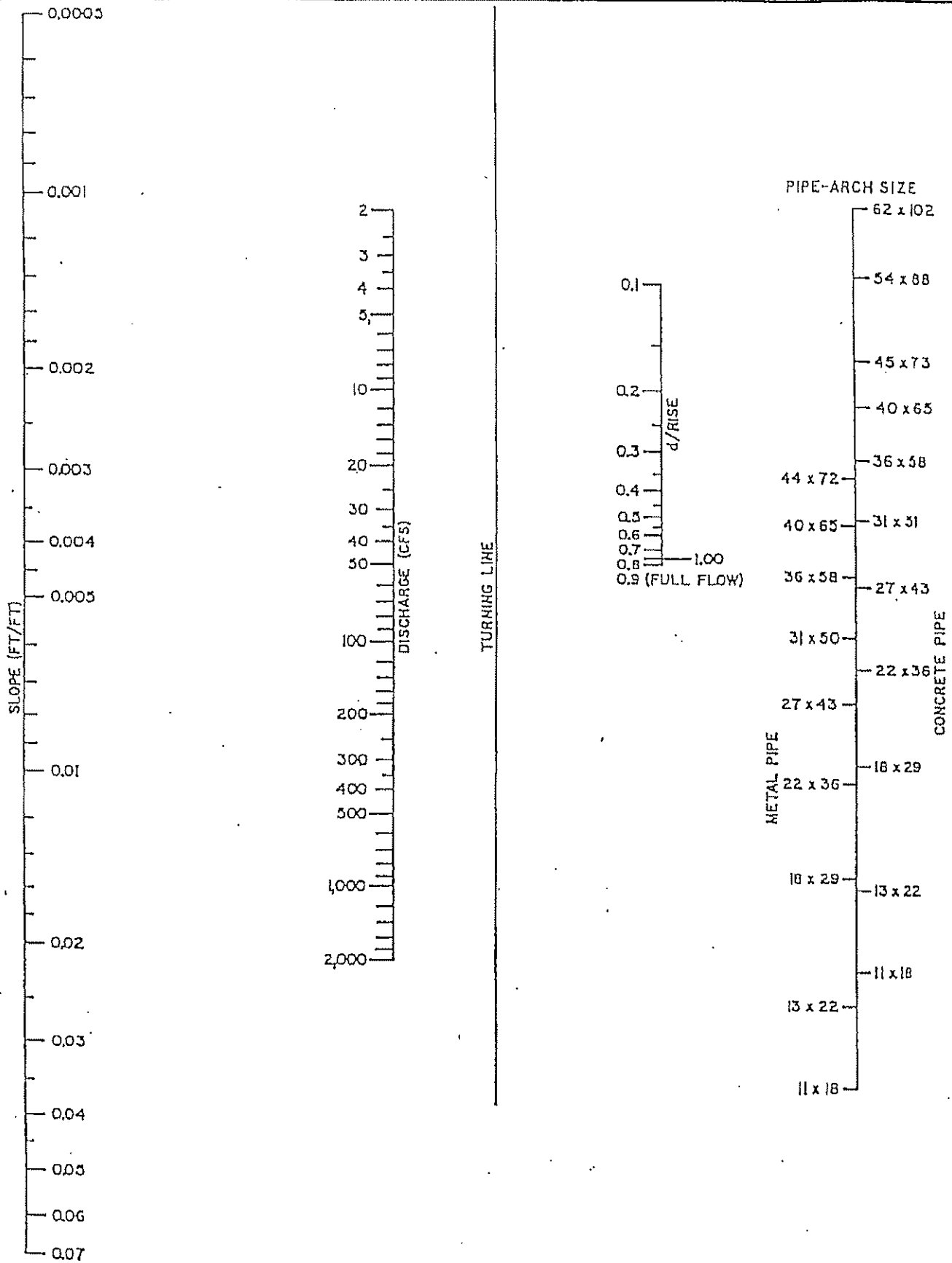
UNIFORM FLOW FOR ARCH PIPE
