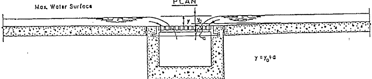
SECTION A-A DROP INLET (Grate covering) Type A-5
