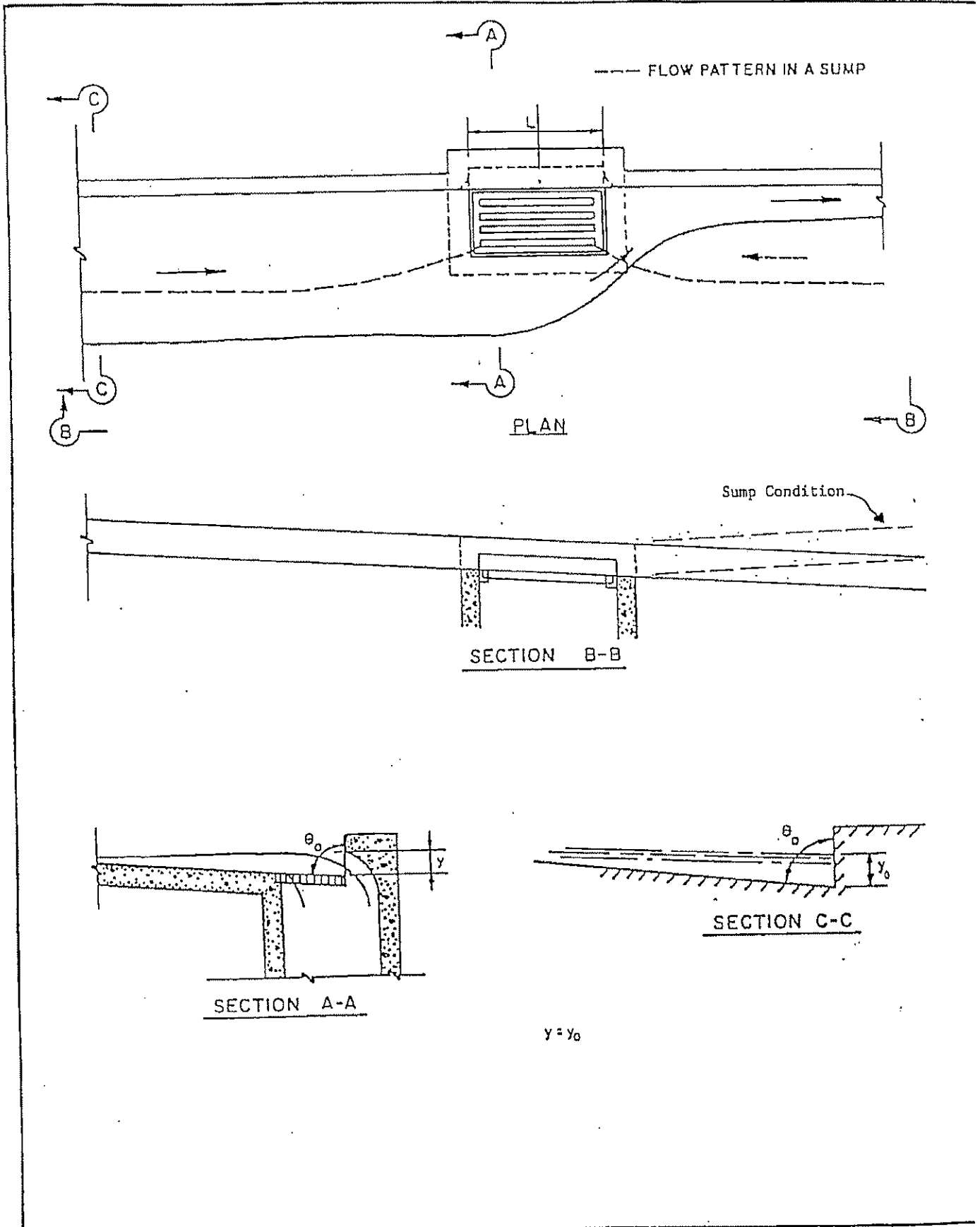
UNDEPRESSED COMBINATION INLET TYPE A-3 & B-3 (RECESSED)
